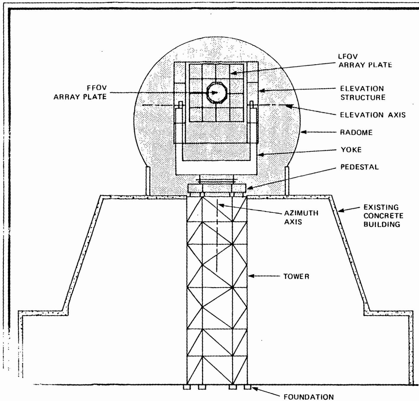
Ground-Based Radar Schematic
